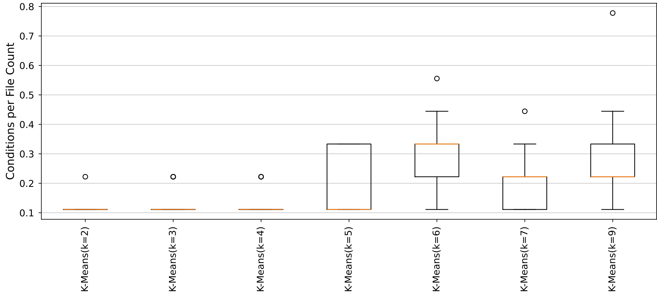
YARA Rules Conditions per File Count Distribution (Cluster13_Size9 dataset)
